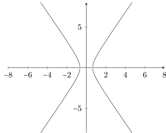
Figure 5.1: 21x^2 - 7y^2 = 9
